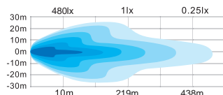
Combo Beam
