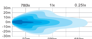
Combo Beam
