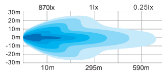
Combo Beam
